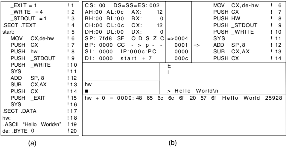
Figure C-1. (a) An assembly language program. (b) The corresponding tracer display.
